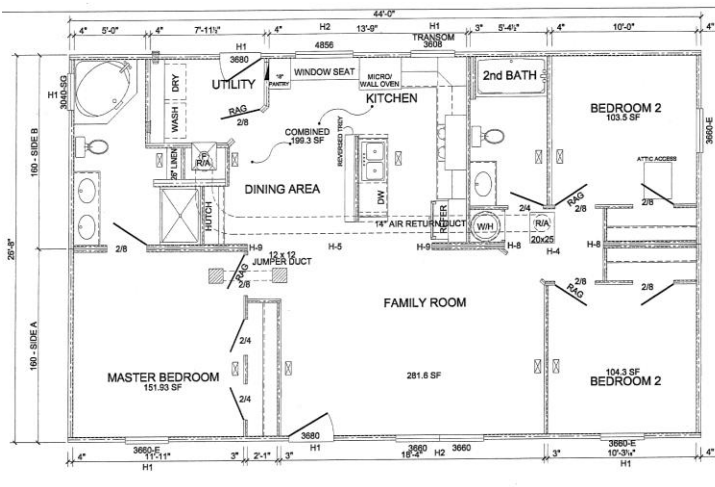
Floor Plan of the New Cottage 6
